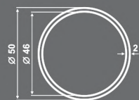
SD-5004 ΚΑΠΑΚΙ ΚΟΛΩΝΑΣ [6m.] Column Cover [6m.]
